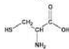
cystein (Cys)
