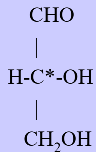
D-glyceraldehyd
