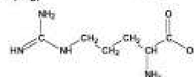
arginin (Arg)
