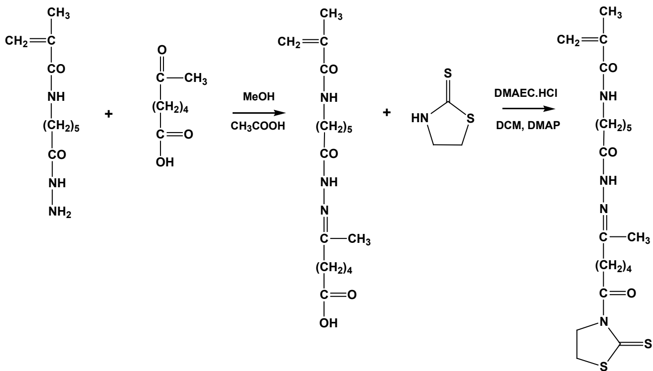
Schema 2. Synthesis of monomer.
