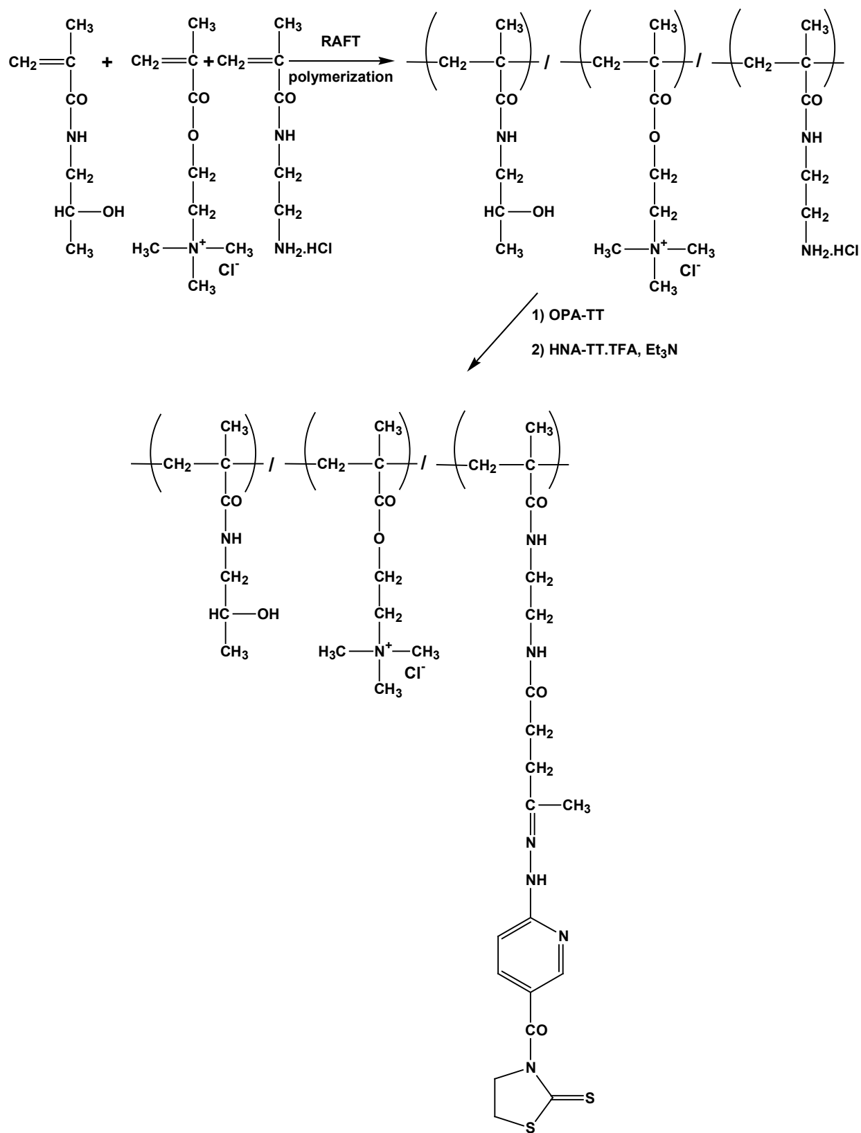
Schema 4. Synthesis of HPMA copolymer with NHA linker and QA groups.
