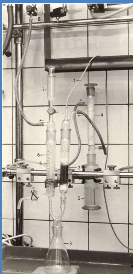
Fig. 2 Heterocontinuous cultivation. The apparatus contains:
