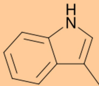
3-methylindol ( skatol )
