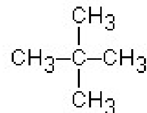
neopentan 2,2-dimethylpropan
