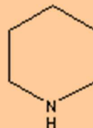
piperidin
