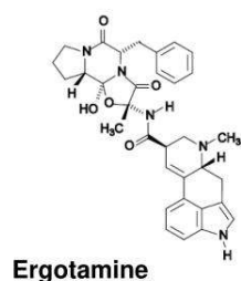
Ergotamine
