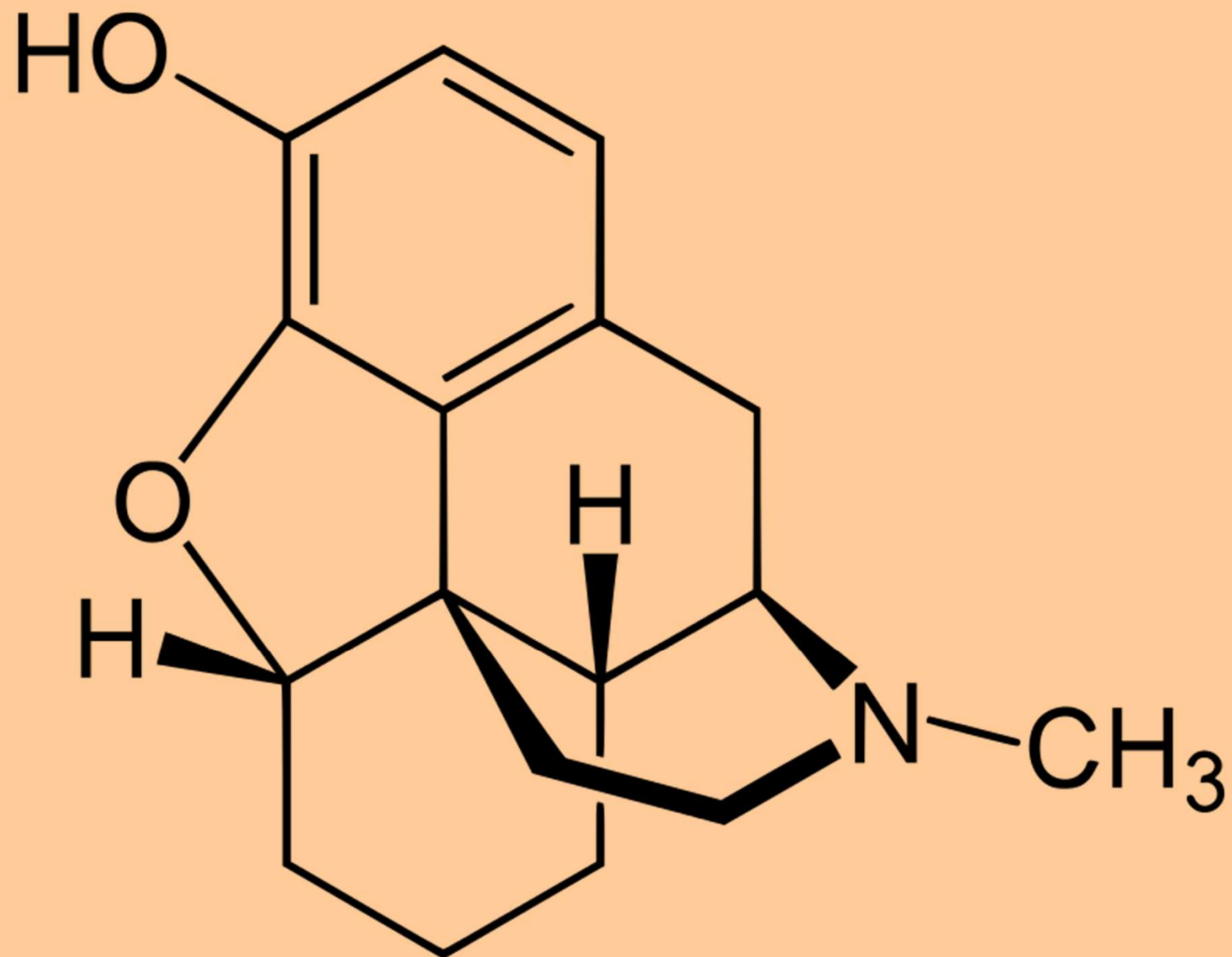
4,5α-epoxy-17-methylmorphinan- 3-ol
