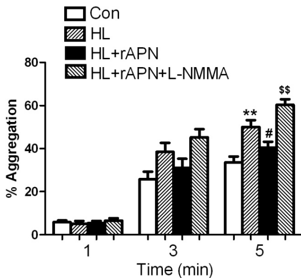
Fig. 1. Effect of rAPN on hyperlipidemia-induced platelet aggregation via turbidimetric method. Con, control; HL, hyperlipidemia; rAPN, recombinant full-length adiponectin; L-NMMA, N G -monomethyl-L-arginine. Values are means \pm S.E.M.; n=5 wells/group. ** P<0.01 vs. Con, # P<0.05 vs. HL. $$ P<0.01 vs. HL+rAPN.
