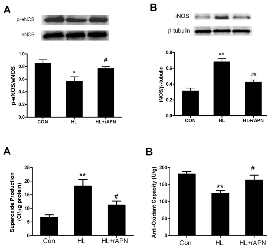
Fig. 4. Effect of rAPN on eNOS phosphorylation and iNOS expression in cultured platelets. A: expression of eNOS and phosphorylated eNOS (p-eNOS; at serine 1177, Western blots) and ratio of p-eNOS/eNOS density analysis. B: representative Western blots and density analysis for iNOS expression. Values are means \pm S.E.M.; n=6 wells of platelets/group. * P<0.05 and ** P<0.01 vs. Con. # P<0.05 and ## P<0.01 vs. hyperlipidemic platelets.
