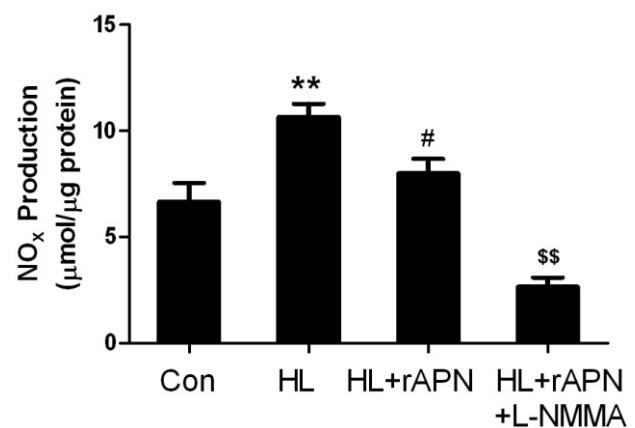
Fig. 3. Total nitric oxide production by platelets isolated from control (Con) or hyperlipidemic blood (HL) treated with vehicle, rAPN (HL+rAPN) or rAPN+L-NMMA (HL+rAPN+L-NMMA). NO concentration in medium containing platelets was determined by Griess reaction. Values are means \pm S.E.M.; n=6 wells of platelets/group. ** P<0.01 vs. Con. # P<0.05 vs. HL. $$ P<0.01 vs. HL+rAPN.
