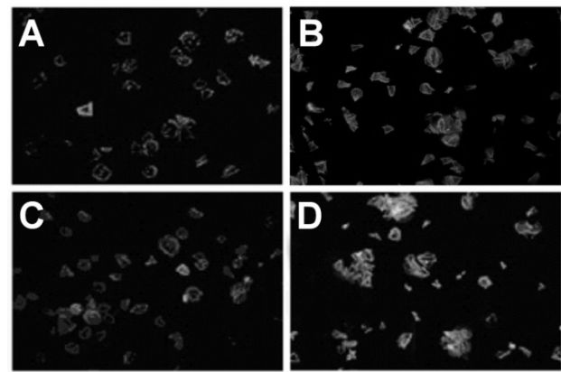
Fig. 2. Effect of rAPN on hyperlipidemia-induced platelet aggregation using immunofluorescence detection. Representative fields of each slide were exhibited in control platelets (A), or hyperlipidemic platelets after treated with vehicle (B), rAPN (C) or rAPN+L-NMMA (D).
