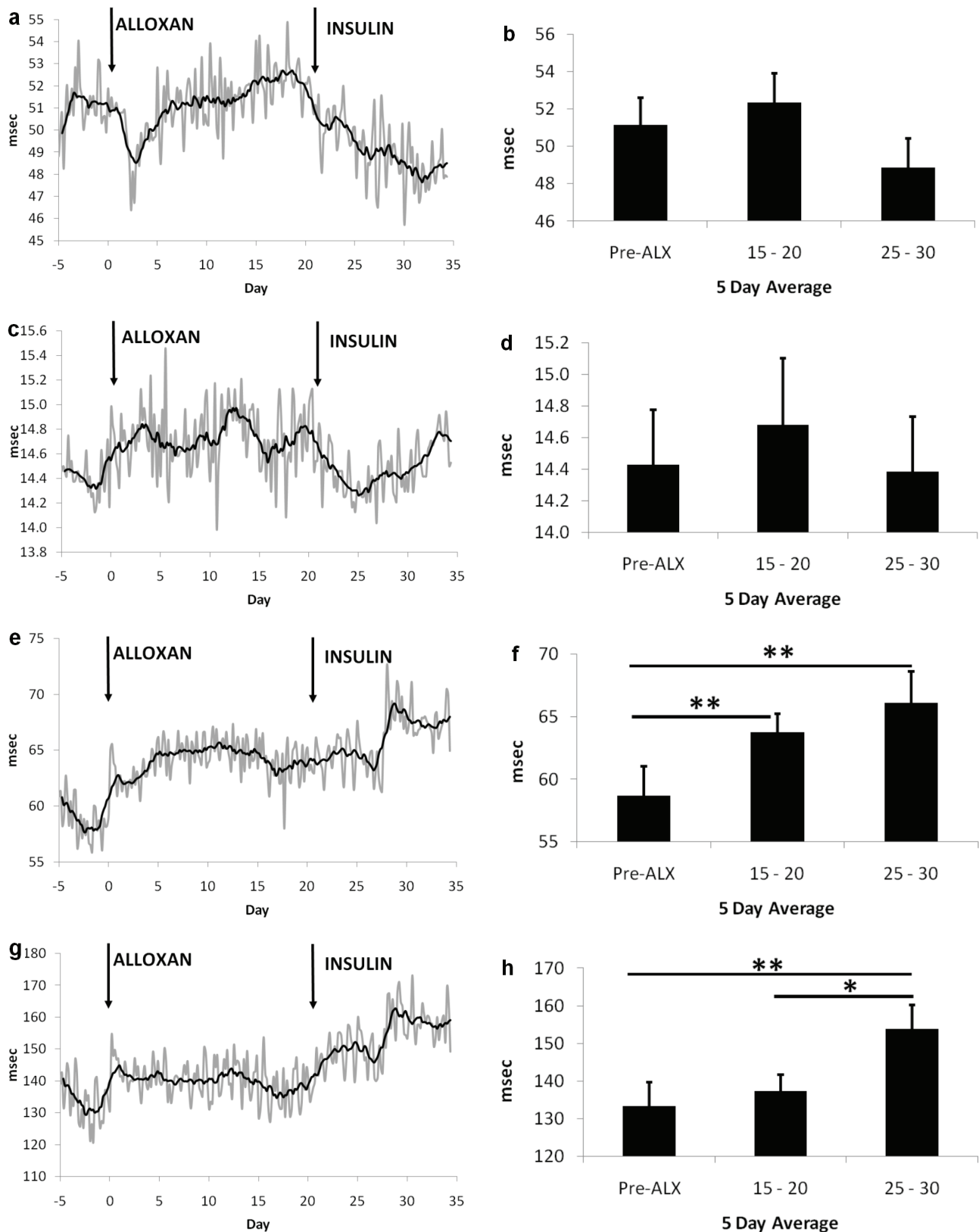
Fig. 3. Effects of ALX-induced diabetes on the electrocardiogram. ( a, c, e, g ) Gray line displays the hourly group mean PQ, QRS, QT and corrected QT intervals, respectively, and black line displays the 24 hr group mean. ( b, d, f, h ) Group mean of PQ, QRS, QT and corrected QT intervals, respectively, with associated standard error bars for pre-ALX, 15-20 days after ALX, and 5-10 days (Day 25-30) following insulin treatment. Data are mean \pm SEM, n=6 rats. Statistical significance * p<0.05 and ** p<0.01 .
