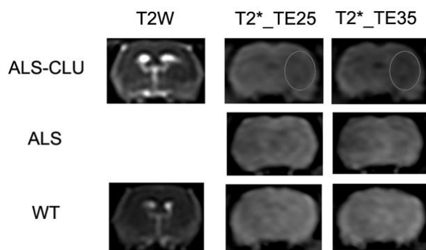
Fig. 1. MRI of the brain of the ALS rat treated with CLUSPIO ("ALS-CLU") as compared to the MRI of the ALS rat without CLUSPIO injection ("ALS") and of the wild type rat ("WT"). T2W protocol reveals the dilated ventricles in the ALS model (images in the left column). T2* protocol reveals the hypointensities (note regions delimited by ellipsoids) allegedly caused by CLUSPIO seen with time to echo (TE) 25 ms (middle column) and further augmented with TE 35 ms (right column).
