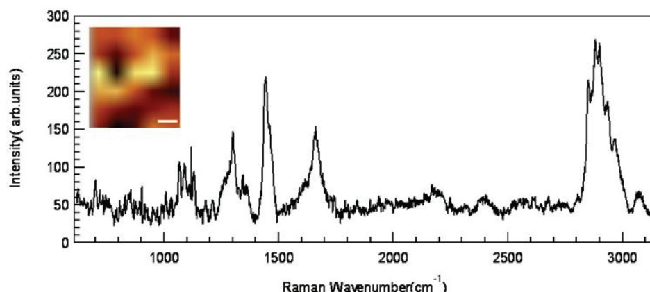
Fig. 5. Raman spectrum extracted from the Raman map image (inset, scale bar 1 \mu\text{m} ) of brain tissue from CLUSPIO treated ALS rats, in the range of 200–3100 \text{cm}^{-1} .
