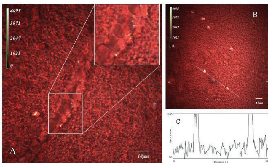
Fig. 2. SECARS image of brain tissue from CLUSPIO treated ALS rats, taken at (A) 2875 cm -1 and (B) at 2850 cm -1 . (C) The corresponding cross section profile shows intensity enhancement along the indicated line shown in the inset of the SECARS image.
