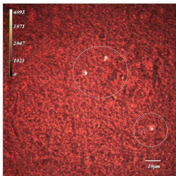
Fig. 3. SECARS image of brain tissue from CLUSPIO- treated ALS rats taken in the finger print region around 1660\text{ cm}^{-1} .
