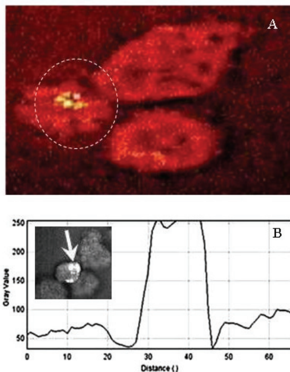
Fig. 4. (A) SECARS image of adipocytes treated with iron oxide nanoparticles (bright regions), taken around 2850\text{ cm}^{-1} . (B) Gray scale plot shows the intensity enhancement highlighting the accumulation of iron oxides nanoparticles indicated by arrow (inset).
