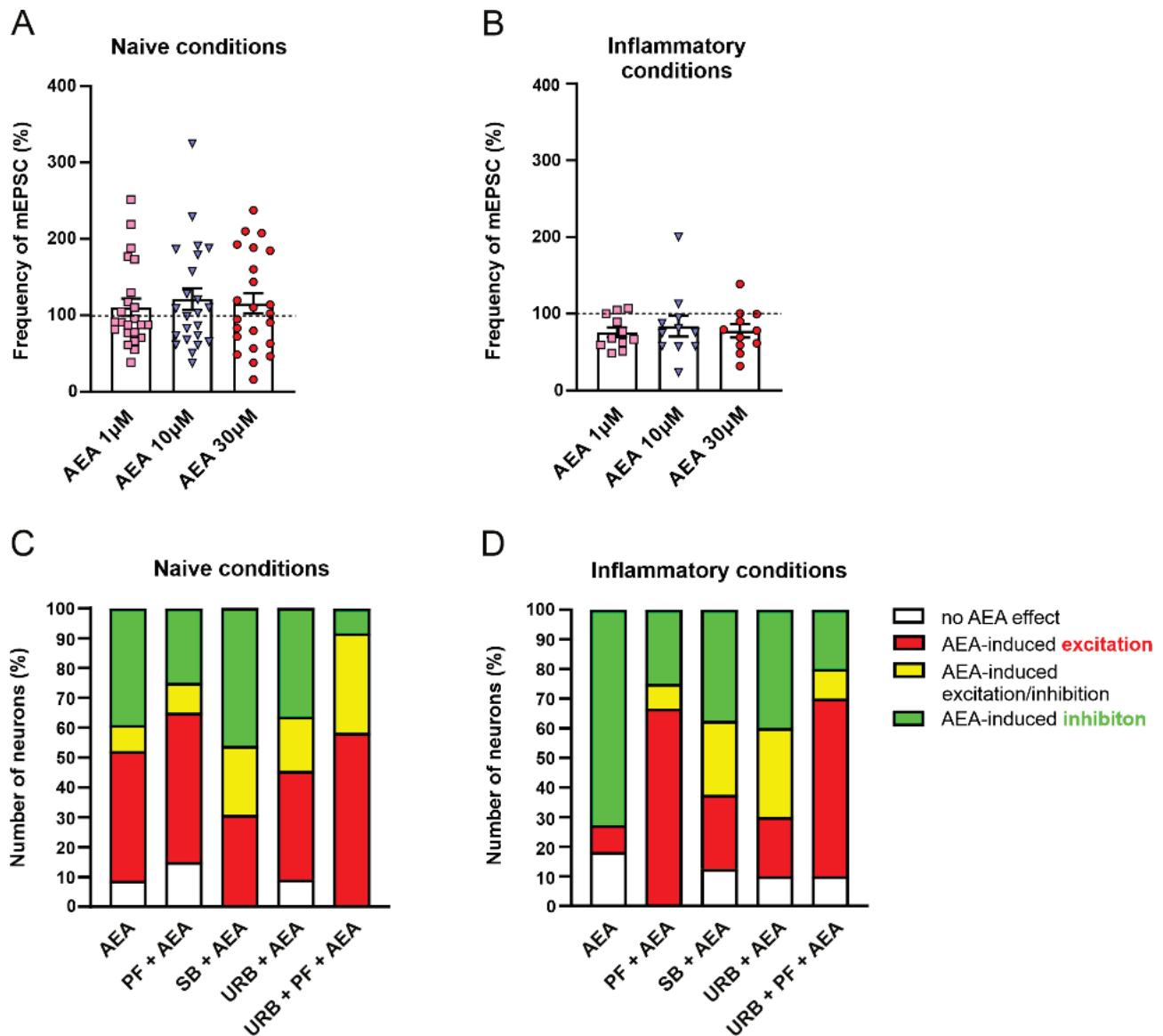
Fig. 3. Peripheral inflammation enhanced the inhibitory effect of AEA application on dorsal horn neurons mEPSC frequency in spinal cord slices. ( A, B ) Normalized frequency of mEPSC during acute AEA application (1 \mu M, 10 \mu M, and 30 \mu M, 4 min each concentration) in control conditions ( A ) and 24 h after induction of peripheral inflammation ( B ) by subcutaneous carrageenan injection. Statistical analysis showed a significant difference between control and inflammatory conditions in each AEA concentration tested (1 \mu M AEA, p < 0.05 ; 10 \mu M AEA, p < 0.05 ; 30 \mu M AEA, p < 0.05 ). ( C ) Application of AEA induced decrease or increase of mEPSC frequency in a comparable number of superficial dorsal horn neurons in control conditions. The number of neurons with mEPSC frequency inhibition by AEA application was reduced after inhibition of the CB 1 receptor (PF514273 application) and especially after CB 1 and FAAH co-inhibition (PF514273/URB597 co-application) used as a pretreatment. ( D ) After peripheral inflammation, most neurons received synaptic input inhibited by the AEA application (73 %). Pretreatment with PF514273 and PF514273/URB597 reduced the inhibitory and enhanced the excitatory AEA-induced effect. Abbreviations: PF (PF514273, CB 1 receptor antagonist), SB (SB366791, TRPV1 antagonist), URB (URB597, FAAH inhibitor). The figure was adapted from Pontearso et al. [10].
