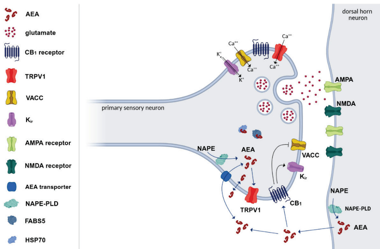
Fig. 2. Simplified illustration of AEA action at the first nociceptive synapse formed by the central terminal of the primary sensory neuron and the secondary spinal cord dorsal horn neuron. Autocrine and retrograde signaling of AEA is suggested, whereas AEA is synthesized in addition to other enzymes by \text{Ca}^{2+} -dependent NAPE-PLD in both primary and secondary nociceptive neurons. (The contribution of glial cells to AEA signaling is not depicted). Translocation of the lipid molecule of AEA across the plasma membrane by diffusion and a membrane transporter was proposed. Intracellular carriers, including the fatty acid binding protein 5 (FABP5) and the heat shock protein 70 (HSP70), may facilitate the intracellular transport of AEA, for example, towards the FAAH for degradation. Two primary AEA-activated receptors are abundantly expressed on the presynaptic side, where they regulate glutamate release. At lower concentrations, the \text{CB}_1 receptor is suggested to be activated, while at higher concentrations, both the \text{CB}_1 and TRPV1 receptors are activated. In addition, AEA could directly inhibit low-voltage-activated calcium channels ( \text{Ca}_v3 ) to modulate the excitability of neuron. The reduction in transmitter release after \text{CB}_1 receptor activation is attributed to the inhibition of high-voltage-activated calcium channels (VACC) and the activation of inwardly rectifying potassium channels ( \text{K}_{\text{ir}} ). The image was created with BioRender.com.
