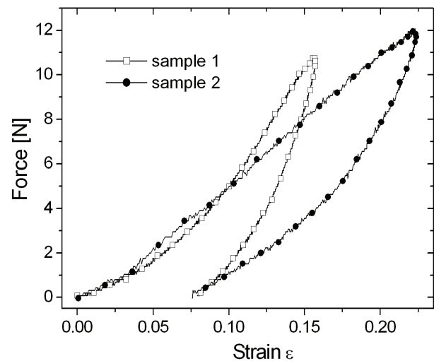
Fig. 3. Examples of loading curves for intact hyaline cartilage tissue from non-weight-bearing zone (sample 1) and cartilage from the defect zone (sample 2). Preload of 1N was considered.
