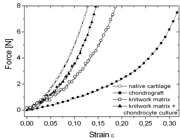
Fig. 7. Loading curves of native cartilage and some of the materials tested: native cartilage sample (the same as in Fig. 2), fibrin chondrograft used for autologous chondrocyte transplantations, knitted chirlac fiber matrix – blank damped in physiological solution and the same chondrocyte-seeded matrix after a ten-day cultivation.
