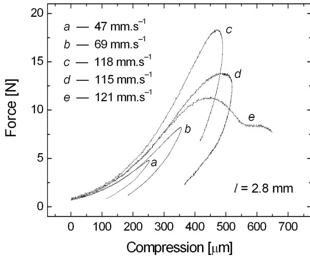
Fig. 4. Force-compression loading curves of single hyaline joint cartilage sample - consequent measurements a to e taken in intervals of 5–10 s. The initial impact velocities v_1 are denoted for each measurement. Uncompressed sample thickness l = 2.8 mm.
