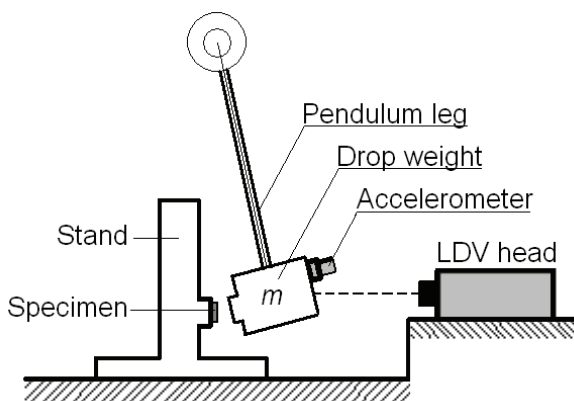
Fig. 1. Scheme of impact loading measurement setup.
