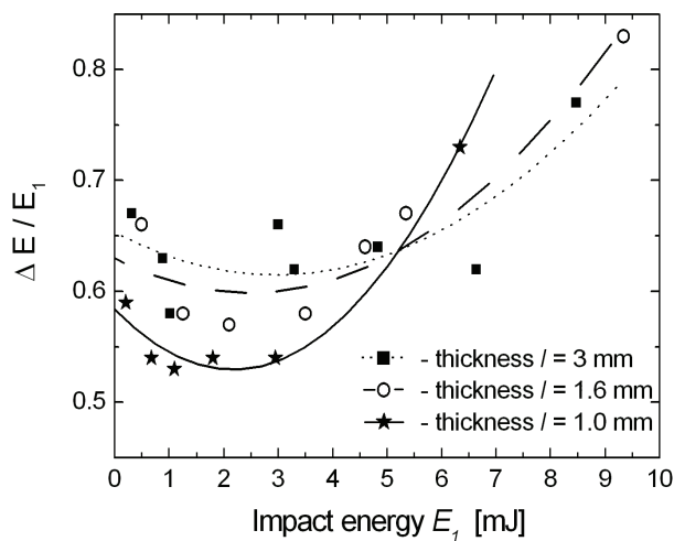
Fig. 6. Dissipation of the impact energy vs. overall impactor energy for three native cartilage specimens. Quadratic fit is shown for each sample data set. Thickness / of individual samples is denoted.
