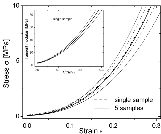
Fig. 2. Stress-strain curves of single cartilage sample and 5 different samples of native pig joint cartilage, mean values and 2 standard deviations confidence intervals. Inset: Tangent modulus nonlinear dependency on actual strain, mean value for single cartilage sample with 2 standard deviations interval.
