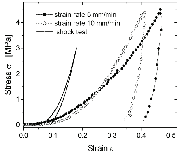
Fig. 5. Comparison of single pig joint cartilage sample stress-strain curves for static (strain rate 5 mm/min and 10 mm/min) and impact (shock test) loading.
