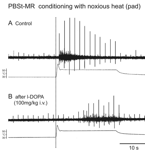
Fig. 1. Depression of the early component of noxious heat induced facilitation of the monosynaptic reflex of PBSt by L-DOPA. (A) control, (B) 80 min after L-DOPA (100 mg/kg i. v.). Anaemically decapitated, high spinalised cat; monosynaptic reflexes evoked by electrical stimulation of the PBSt nerve (stimulus strength 5 times threshold) recorded from ventral roots L7/S1; noxious radiant heat (52 °C) applied to the central pad of the foot (lower traces in A and B). Modified from Schomburg and Steffens (1998).
