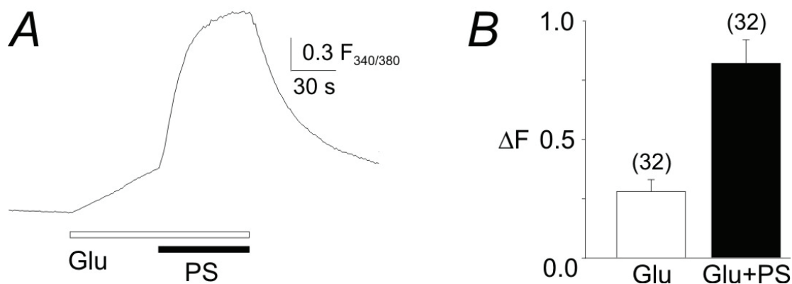
Fig. 1. Agonist-dependent effect of PS. A. A change in the fluorescence ratio ( F_{340/380} ) in a GFP-positive HEK293 cell in a culture transfected by GFP, GluN1, and GluN2B. The response was induced by 0.3 \mu\text{M} glutamate (the duration is indicated by open bar) and its co-application with 300 \mu\text{M} PS (indicated by filled bar). Glutamate and the neurosteroid were applied in the ECS containing 1 % DMSO, 20 \mu\text{M} glycine, 2 mM \text{Ca}^{2+} , and no added \text{Mg}^{2+} . B. Bar graph summarizes the relative changes in the fluorescence ( \Delta F ) induced by 0.3 \mu\text{M} glutamate (Glu) and its co-application with 300 \mu\text{M} PS (Glu + PS). The relative changes in the fluorescence induced by glutamate application were calculated from \Delta F = F_{\text{Glu}} - F_0 , where F_0 is the fluorescence intensity ratio at 340 and 380 nm before the start of test solution application and F_{\text{Glu}} is the fluorescence ratio at the end of glutamate application. In the case of glutamate and PS, co-application the fluorescence was calculated from \Delta F = F_{(\text{Glu}+\text{PS})} - F_0 , where F_{(\text{Glu}+\text{PS})} is the fluorescence ratio at the end of glutamate and PS co-application. Error bars represent mean \pm SEM, and the number of cells studied is indicated in parentheses. There is a statistically significant difference between \Delta F induced by glutamate and its co-application with PS (Mann-Whitney: P=0.002 ).
