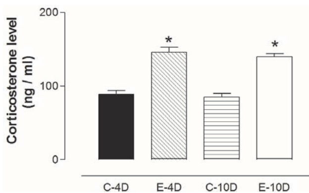
Fig. 4. Plasma corticosterone level at rest (C-4D, n = 10 ; C-10D, n = 10 ), immediately after the fourth day (E-4D, n = 10 ), and the tenth day (E-10D, n = 10 ) of exercise. * indicates significant difference ( P < 0.05 ) in comparison with control values.
