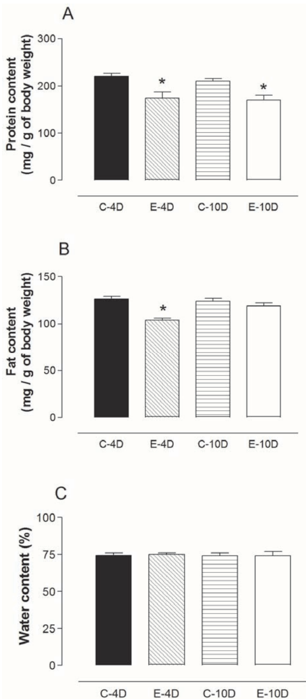
Fig. 2. Effect of IE on body chemical composition of C-4D (n=10), C-10D (n=10), four-day exercised (E-4D, n=10), and ten-day exercised (E-10D, n=10) animals. Levels of protein (A), fat (B) and water (C) content, respectively. * indicates significant difference ( P < 0.05 ) in comparison with correspondent control group.
