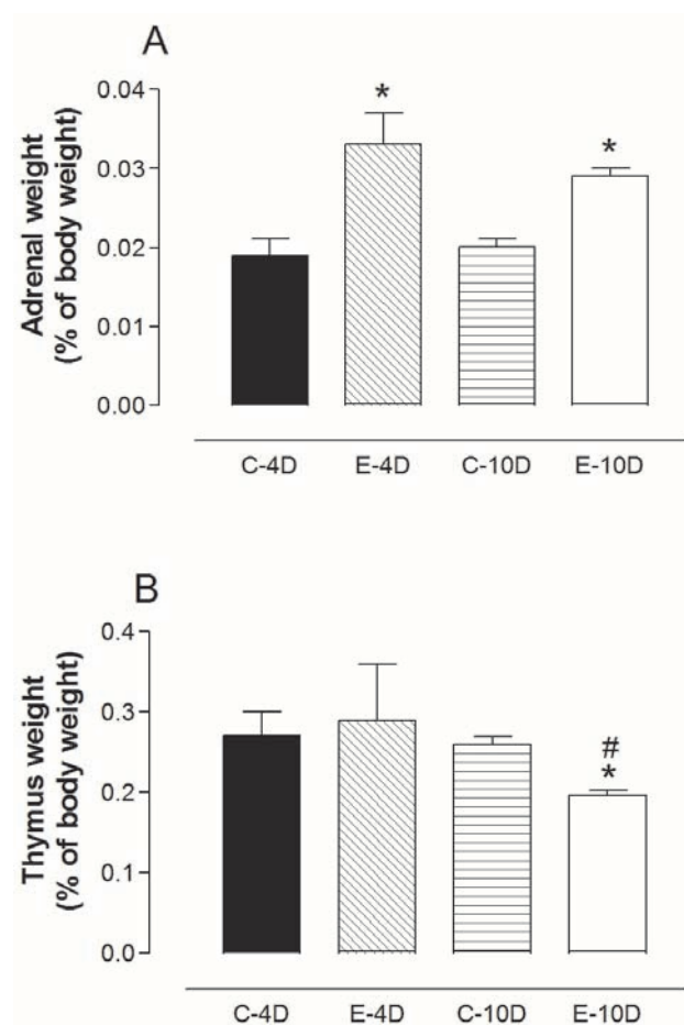
Fig. 5. Weight of adrenal (A) and thymus (B) glands, expressed as percentage of body weight in C-4D, C-10D, four-day exercised (E-4D), and ten-day exercised (E-10D) animal groups ( n = 10 for the four groups). * indicates significant difference ( P < 0.05 ) in comparison with correspondent significant control group and # in comparison to E-4D group.
